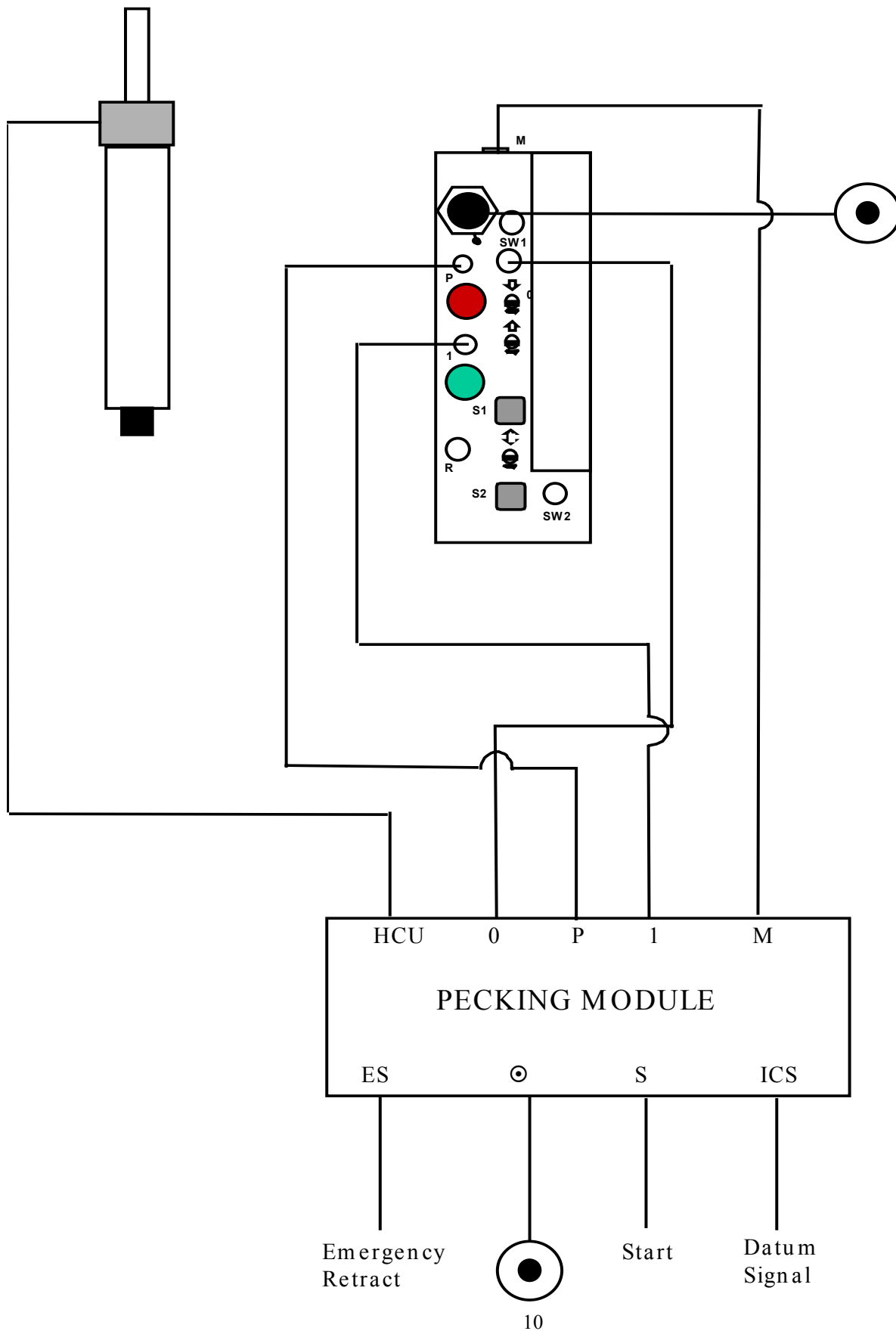
Connection Diagram
