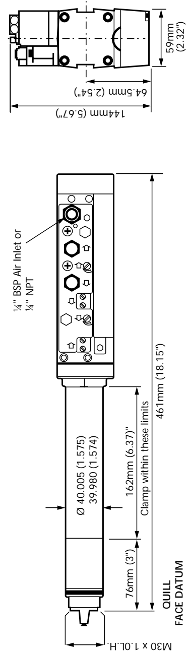
AFD215 pneumatic drive
