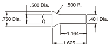
CHISEL SHANK DIMENSIONS
