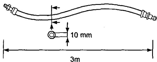
Recommended inlet hose
