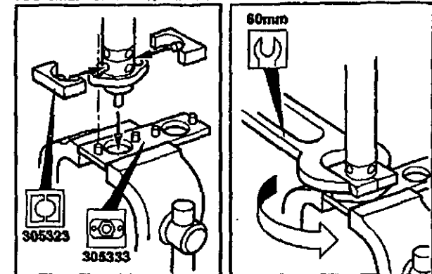
To Dismantle: Refer to main illustration
