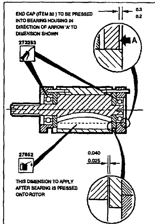
To Assemble: Motor complete, refer to main illustration
