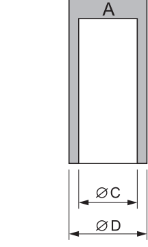
Dismantling tool Mandrel A
