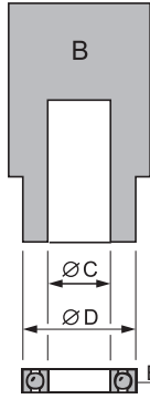
Assembly tool Mandrel B
