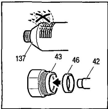
UNCOOLED FRONT SEALED AIR FLOW
