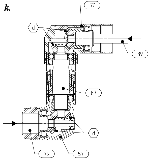
(remontage M180)
